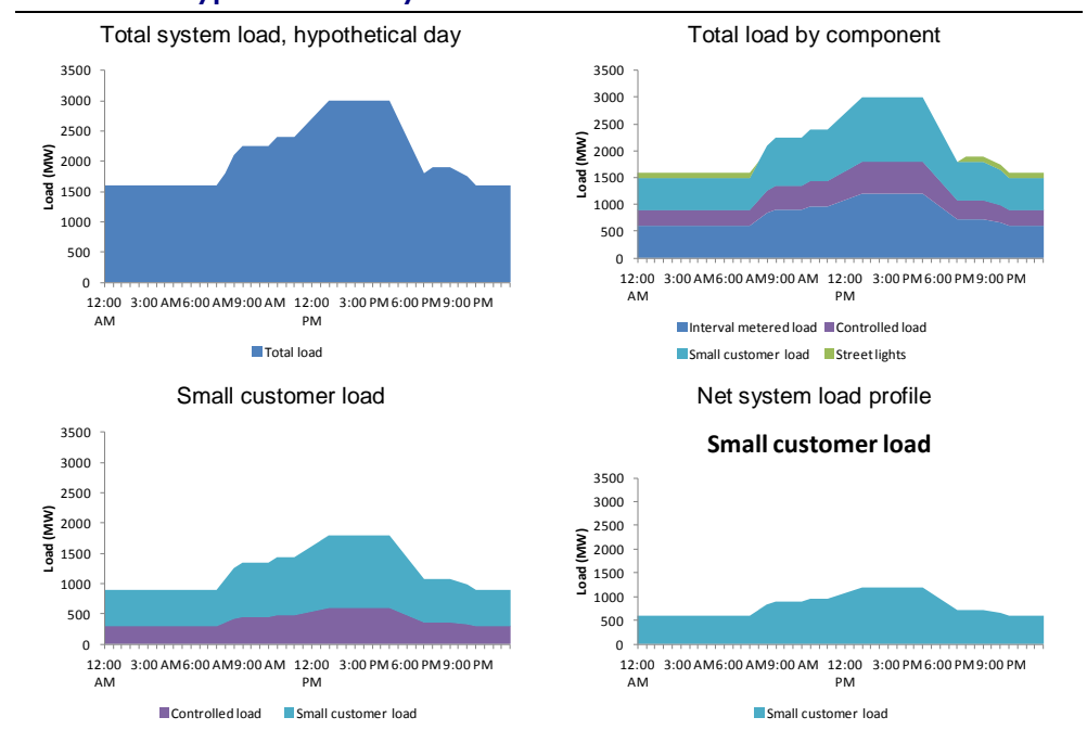
Figure 1 Example of developing the Net System Load Profile for a hypothetical day
